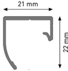
Winkel-Clip 50°/60°
